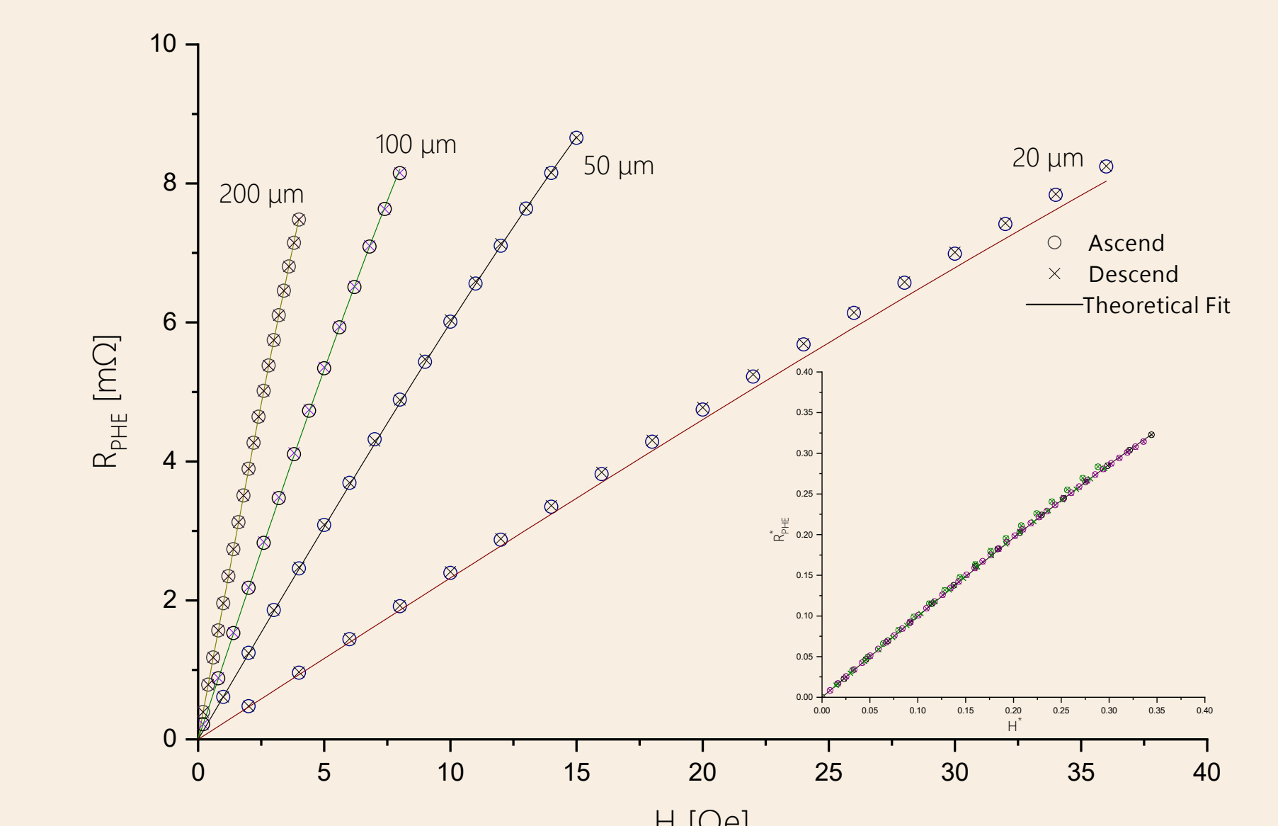
Figure 2. Operational field ranges for sensors with different hard axis lengths. The inset presents scaled data with normalized values.
